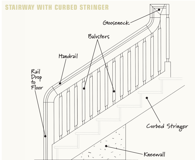
With a curbed stringer, the ends of the risers and treads are not visible from the side.
